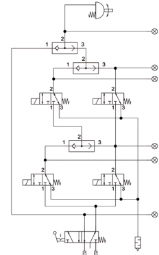
2oo3 (Two out of Three)
